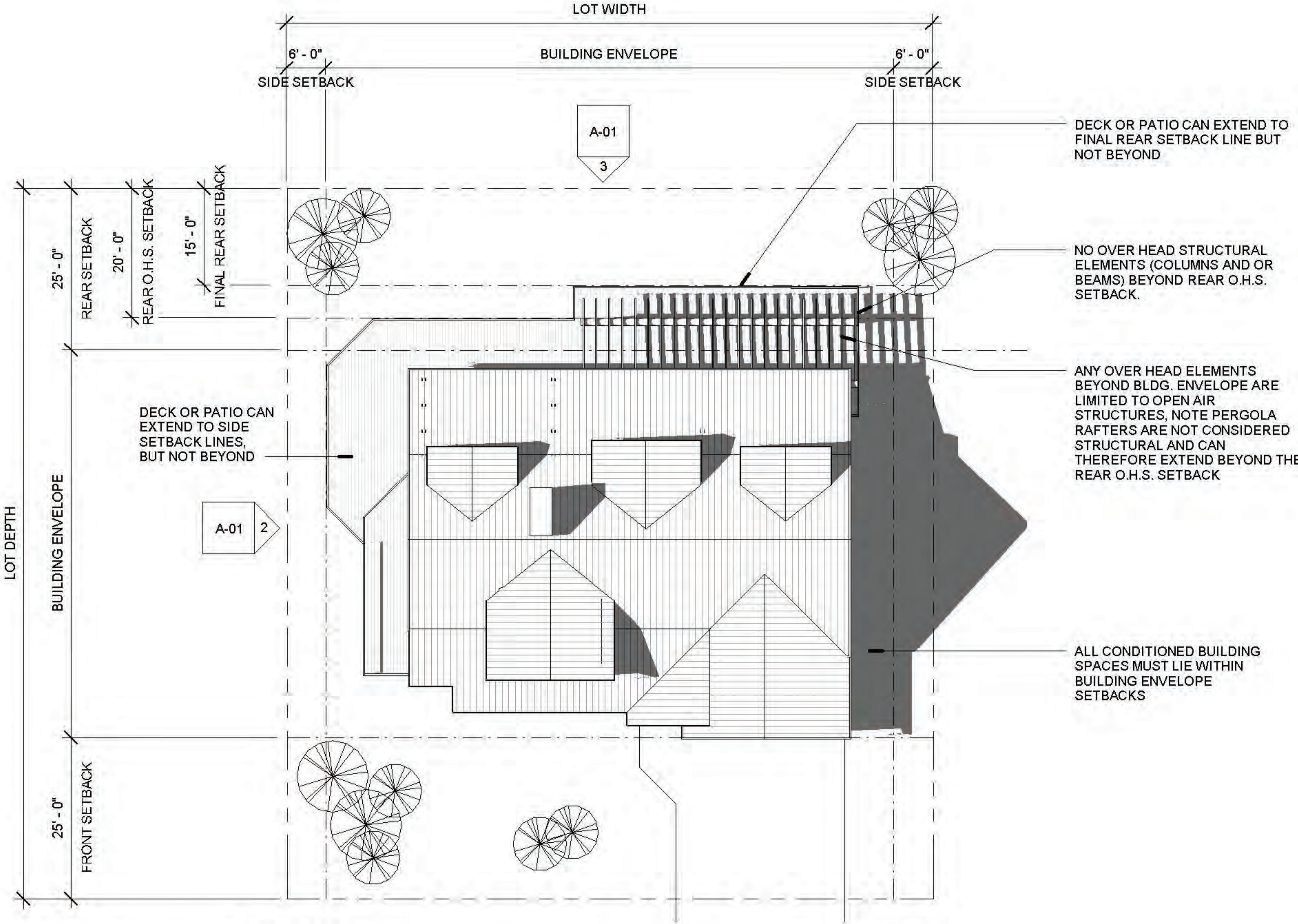
1 SITE PLAN 1/16" = 1'-0"
